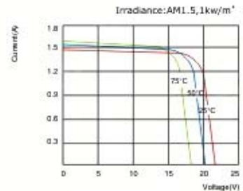
SLP025-12 I-V Curves
